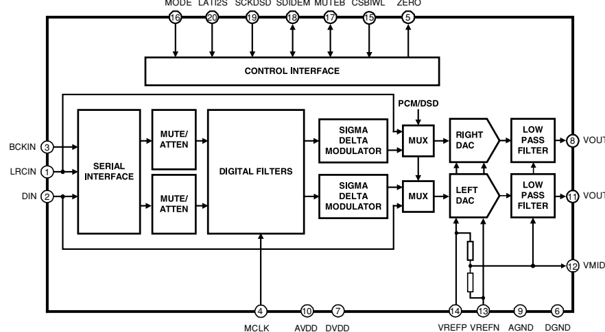
IC603: WM8728 24-bit, 192 kHz stereo DAC
