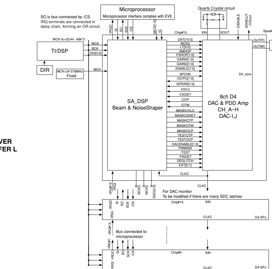
IC601, 602: YDA141-SZ Sound projector
